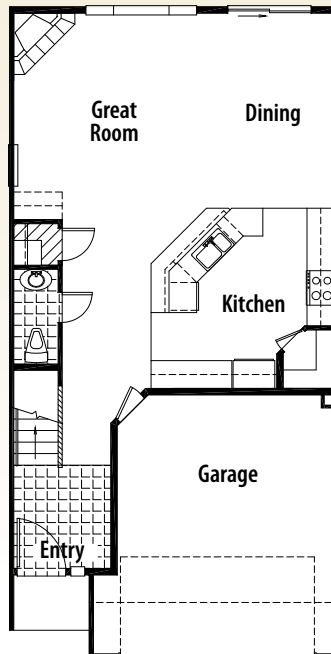
MAIN FLOOR 768 Square Feet
